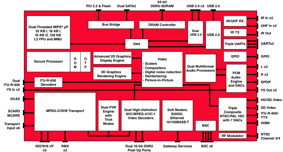
BCM7400 Block Diagram
